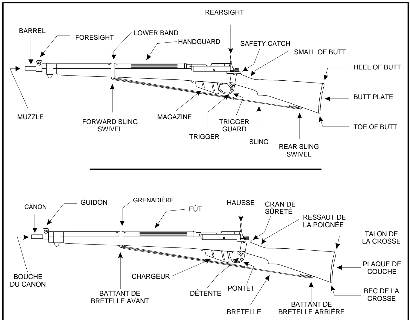
Figure 2-1 Parts of the rifle Figure 2-1 Parties du fusil
