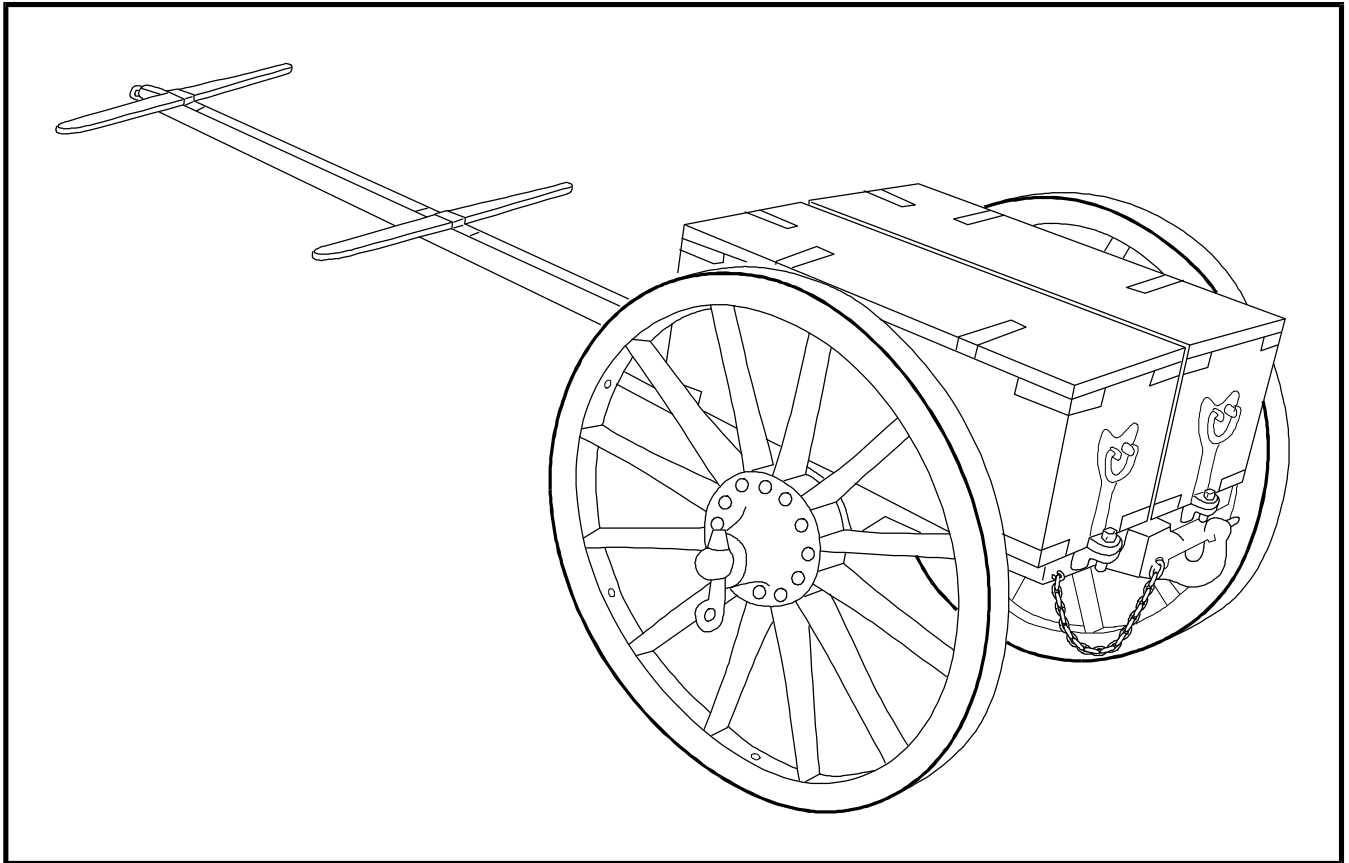
Figure 4-2 Carriage and limber Figure 4-2 Affût et avant-train
